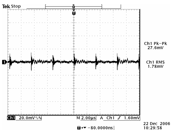
Ripple and noise at no load, 76 Vdc input
