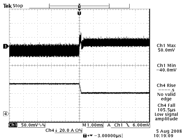
75%-50% Load Transients at Vin=48 V, Vo=3.3 V
