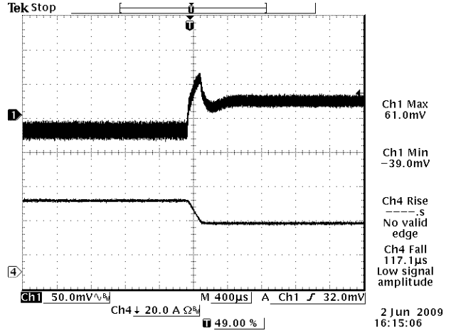
75%-50% Load Transients at Vin=48 V, Vo=1.2 V
