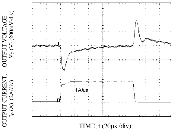
Transient Response to Dynamic Load Change from 0% to 50% to 0%. V_o=1.8V
