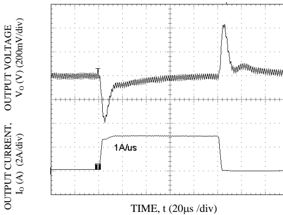
Transient Response to Dynamic Load Change from 0% to 50% to 0%. V_o=3.3V
