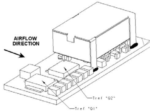
Preferred airflow direction and location of hot-spot of the module ( T_{ref} ).
