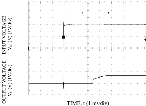
Start-up Using Input Voltage ( V_{IN} = 10V , I_o = I_{o,max} ), V_o = 0.69V
