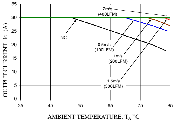
Vo=1.8V, Vin=12V
