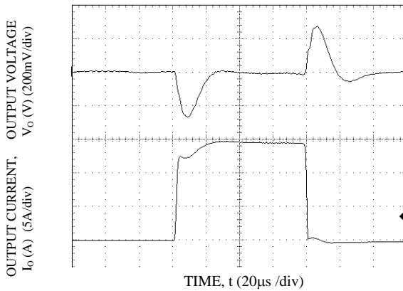
Transient Response to Dynamic Load Change from 0% to 50% to 0%. V_o=1.8V , T_a=25^\circ C , V_{in}=12V
