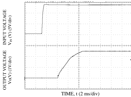
Start-up Using Input Voltage ( V_{IN} = 14V , I_o = I_{o,max} ), V_o = 2.5V , T_a = 25^\circ C
