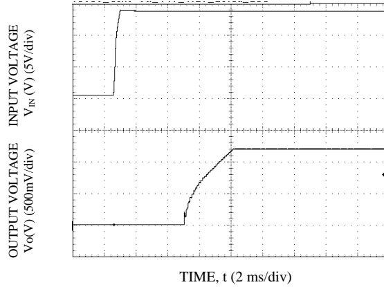
Start-up Using Input Voltage ( V_{IN} = 14V , I_o = I_{o,max} ), V_o = 1.2V , T_a = 25^\circ C
