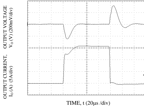
Transient Response to Dynamic Load Change from 0% to 50% to 0%. V_o=1.2V , T_a=25^\circ C , V_{in}=12V
