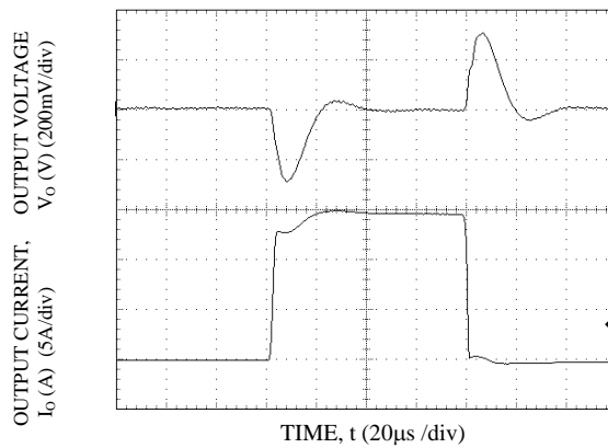
Transient Response to Dynamic Load Change from 0% to 50% to 0%. V_o=2.5V , T_a=25^\circ C , V_{in}=12V
