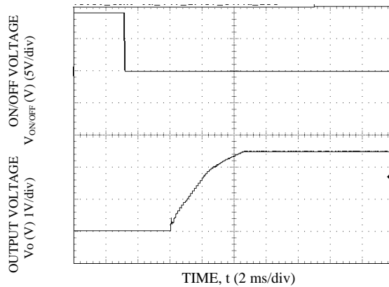
Start-up Using On/Off Voltage ( I_o = I_{o,max} ) V_o=2.5V , T_a=25^\circ C
