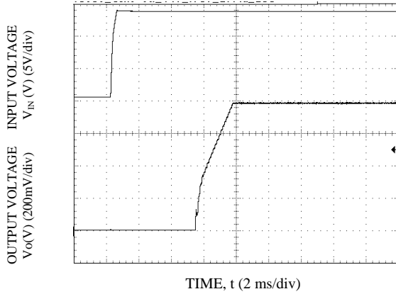
Start-up Using Input Voltage ( V_{IN} = 14V , I_o = I_{o,max} ), V_o = 0.8V , T_a = 25^\circ C
