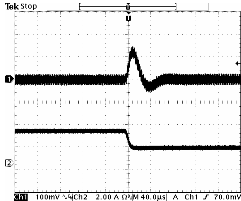
Transients 100% to 50% load 1.8 Vdc output
