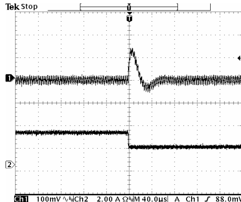
Transients 100% to 50% load 0.75 Vdc output
