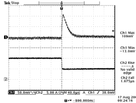
100% to 50% load Transient at Vin=5 V, Vo=0.75 V
