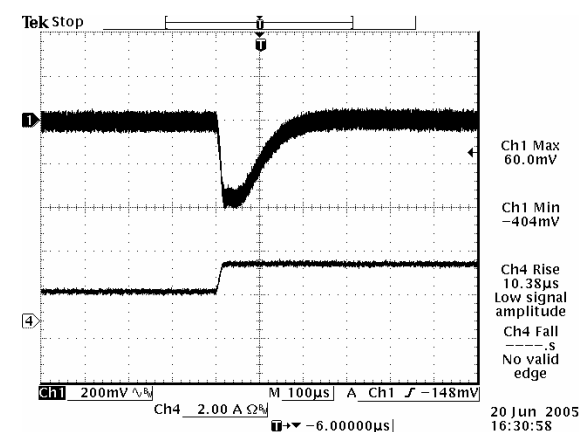
Vo=12 V 25% to 50% Load Transients
