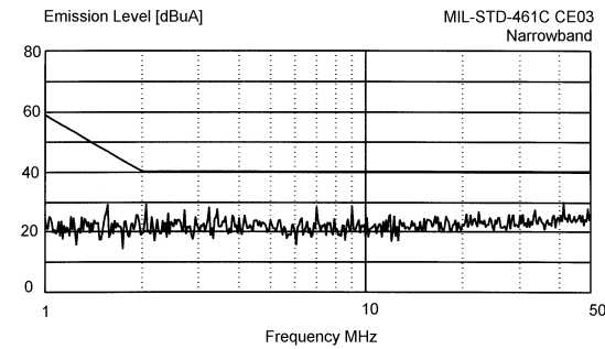
Figure 9 – MIL-STD-461C Two DVTR2800S's With DVMC28 EMI Filter
